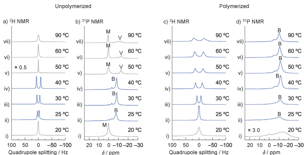
Figure 1. Variable-temperature NMR spectra of bicellar mixtures composed of DMPC and polymerizable surfactants (SC-M 1 and SC-M 3 ) with a molar ratio of DMPC/SC-M 1 /SC-M 3 = 80:19:1 in D 2 O containing 100 mM KCl (total lipid content, 10 % w/v ). a, b) Before polymerization. c, d) After polymerization. 2 H quadrupole splitting (a, c) and 31 P NMR spectra with 1 H decoupling of 6 kHz (b, d) were measured. In the 31 P NMR spectra, M, B, and V indicate signals assignable to micelles, bicelles, and vesicles, respectively.
